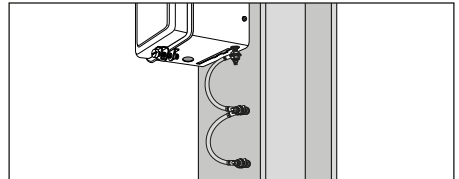
Protective bonding circuit - Double point connection
